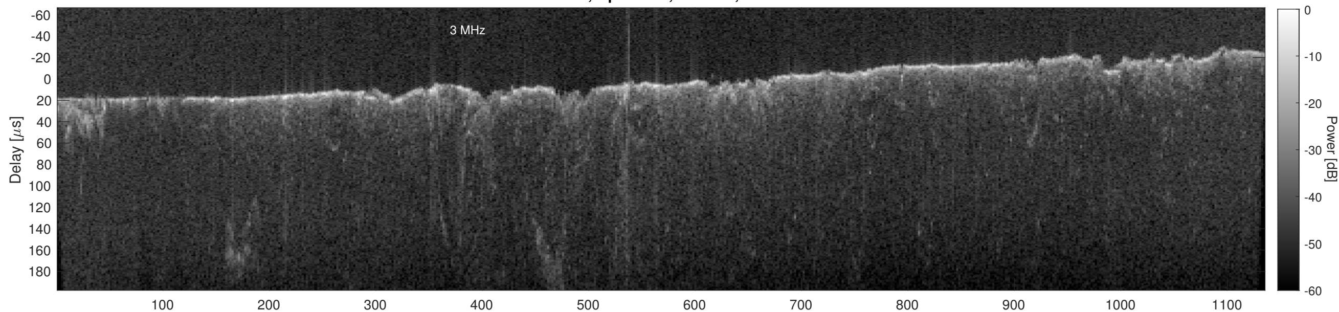
Orbit 17579, Cluttergram
