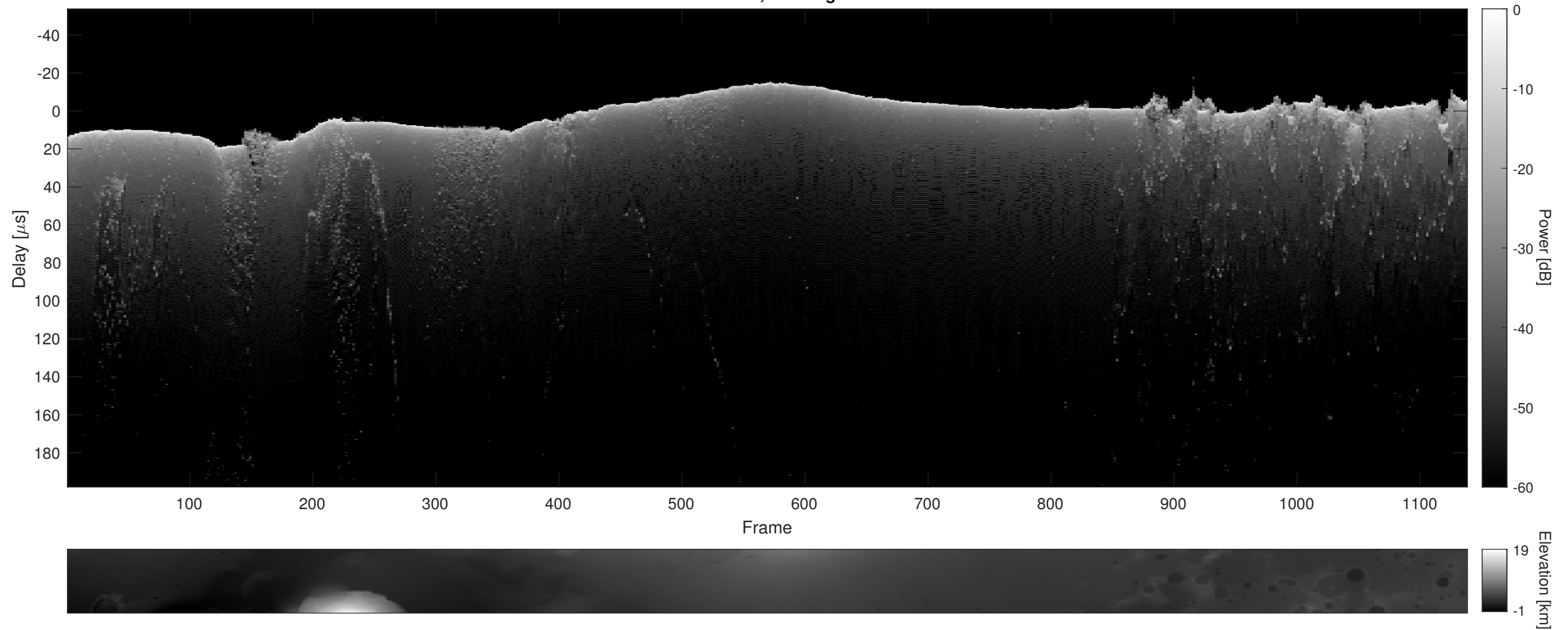
Orbit 17580, Cluttergram
