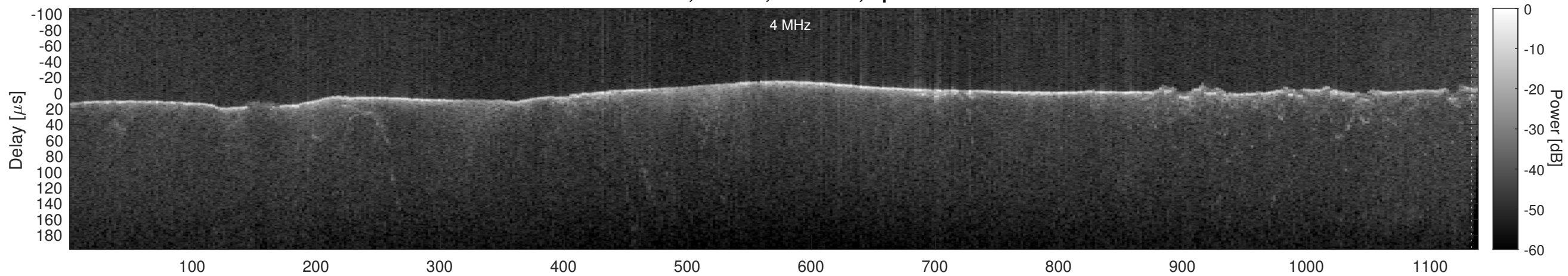
Orbit 17580, Cluttergram
