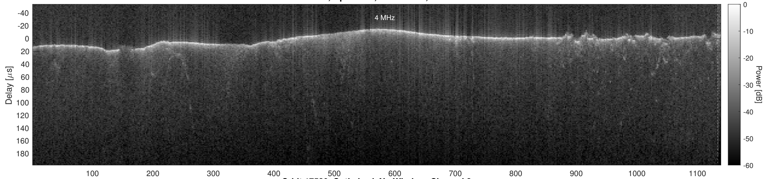
Orbit 17580, Optimized, No Window, Channel 2
