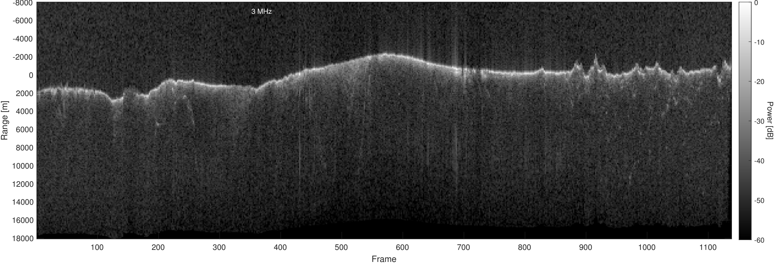
Orbit 17580, Optimized, Window, Depth-Corrected, Channel 2
