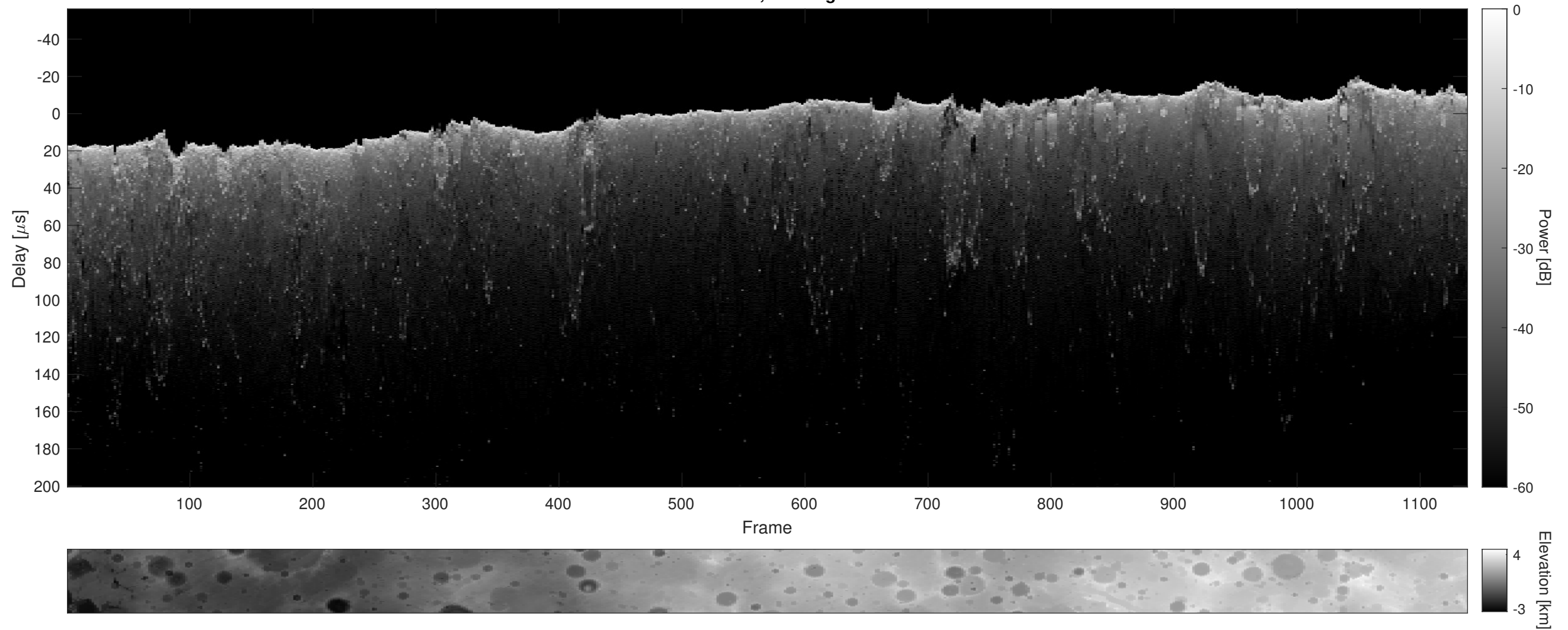
Orbit 17582, Cluttergram
