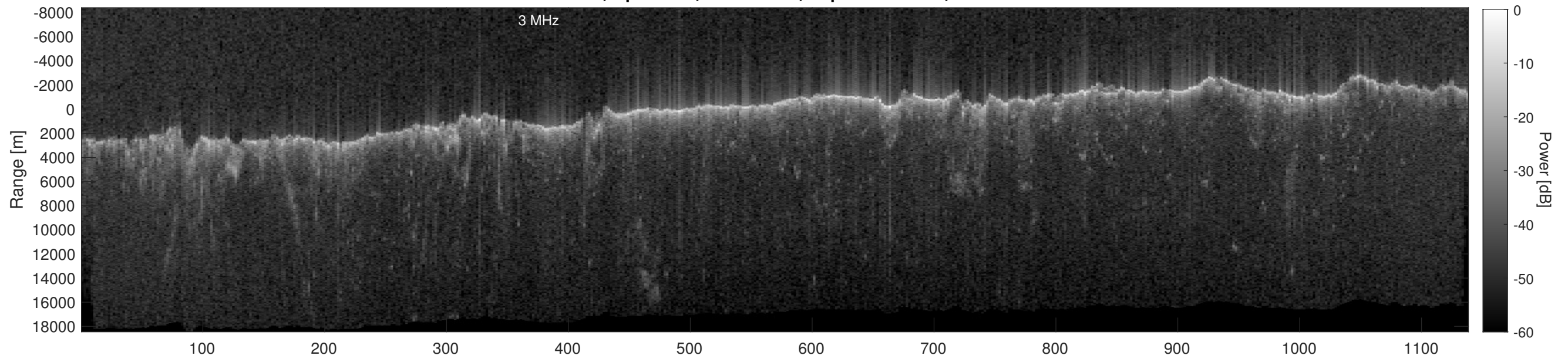
Orbit 17582, Depth-Corrected Cluttergram
