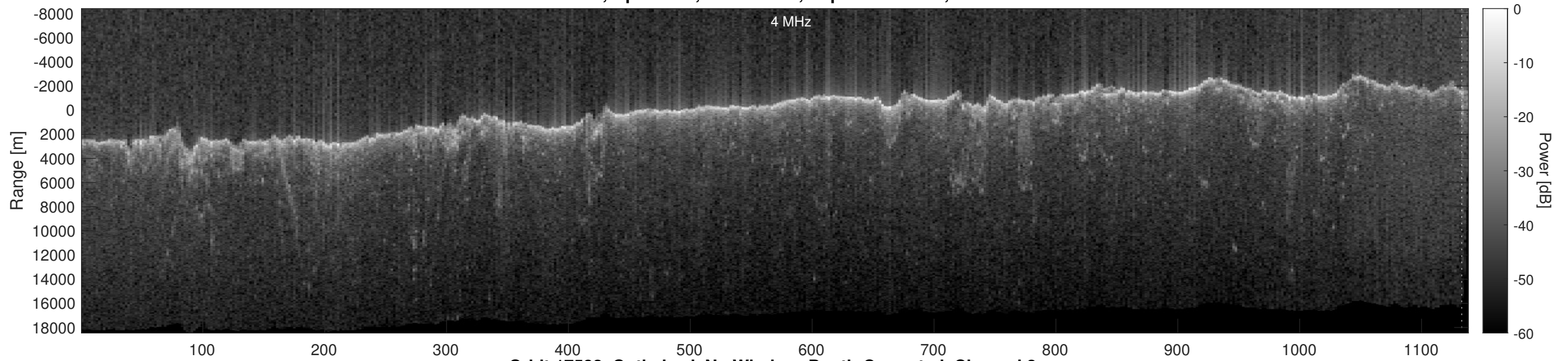
Orbit 17582, Optimized, No Window, Depth-Corrected, Channel 2
