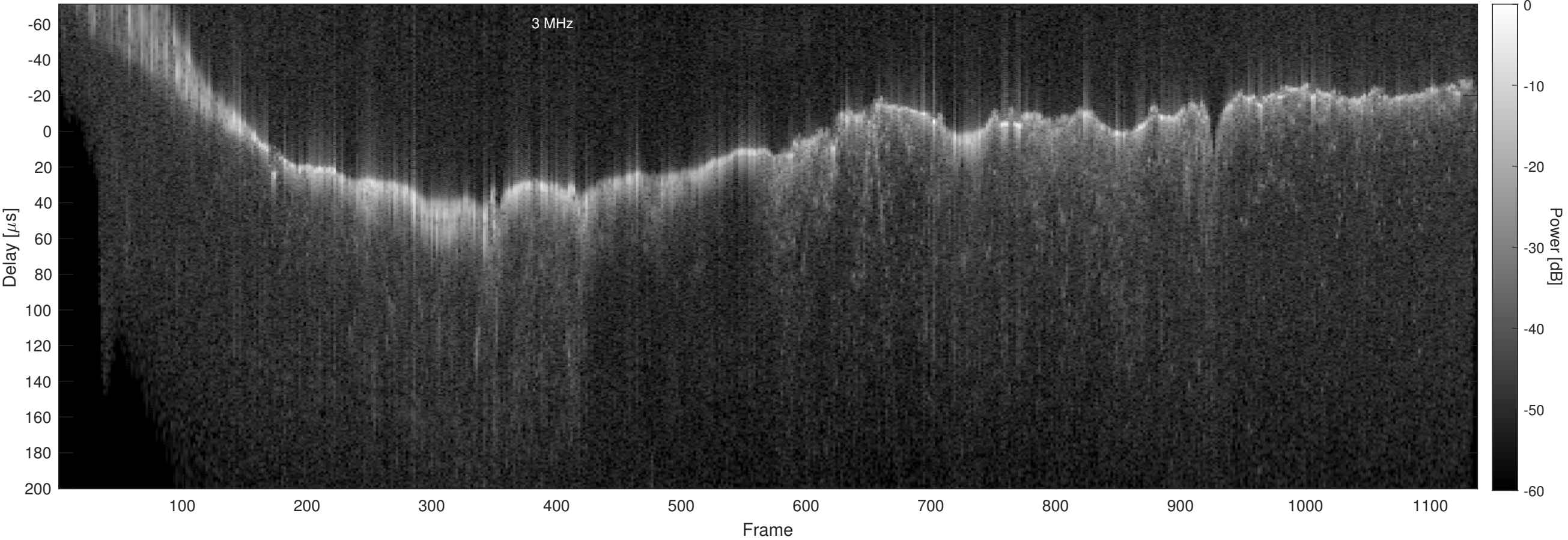
Orbit 17584, Chapman, No Window, Channel 2
