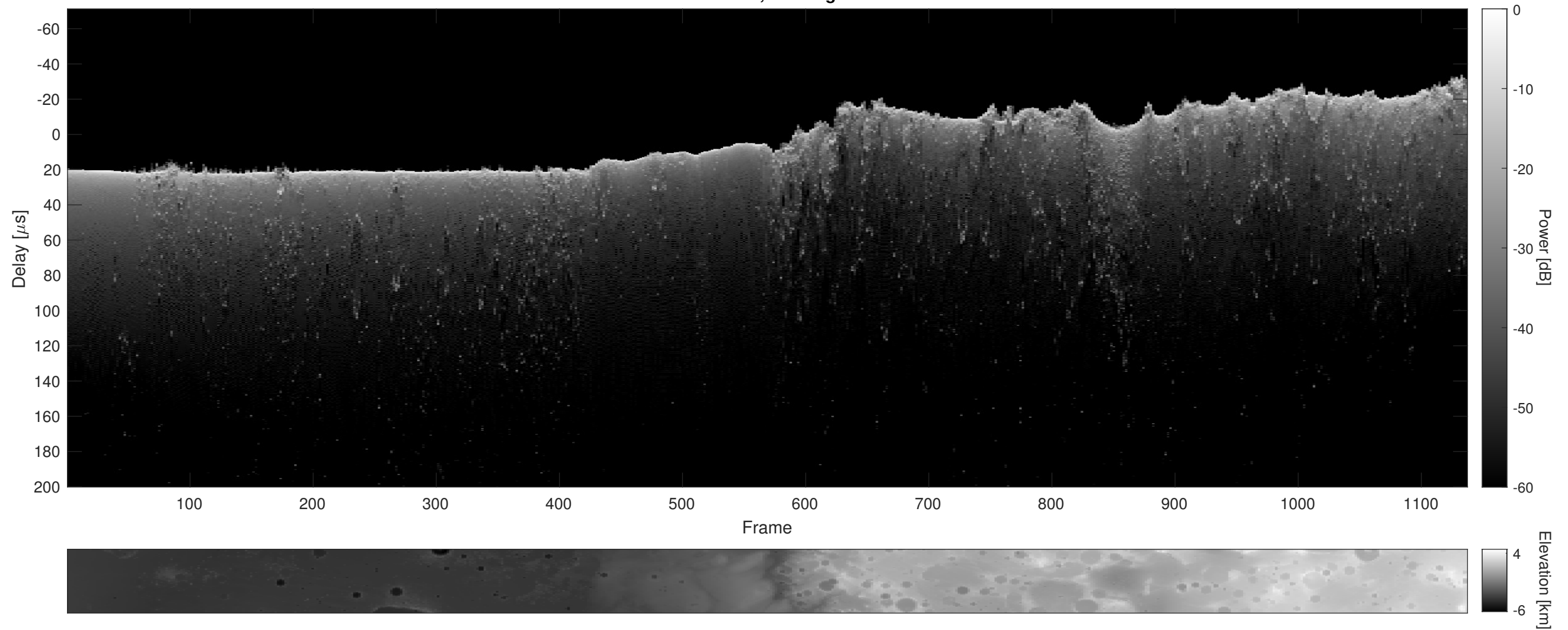
Orbit 17584, Cluttergram
