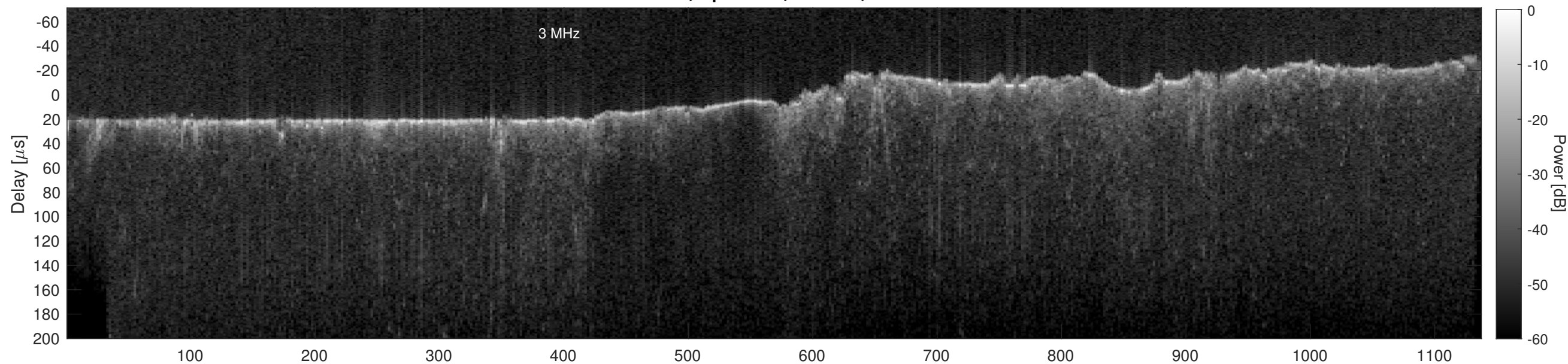
Orbit 17584, Cluttergram
