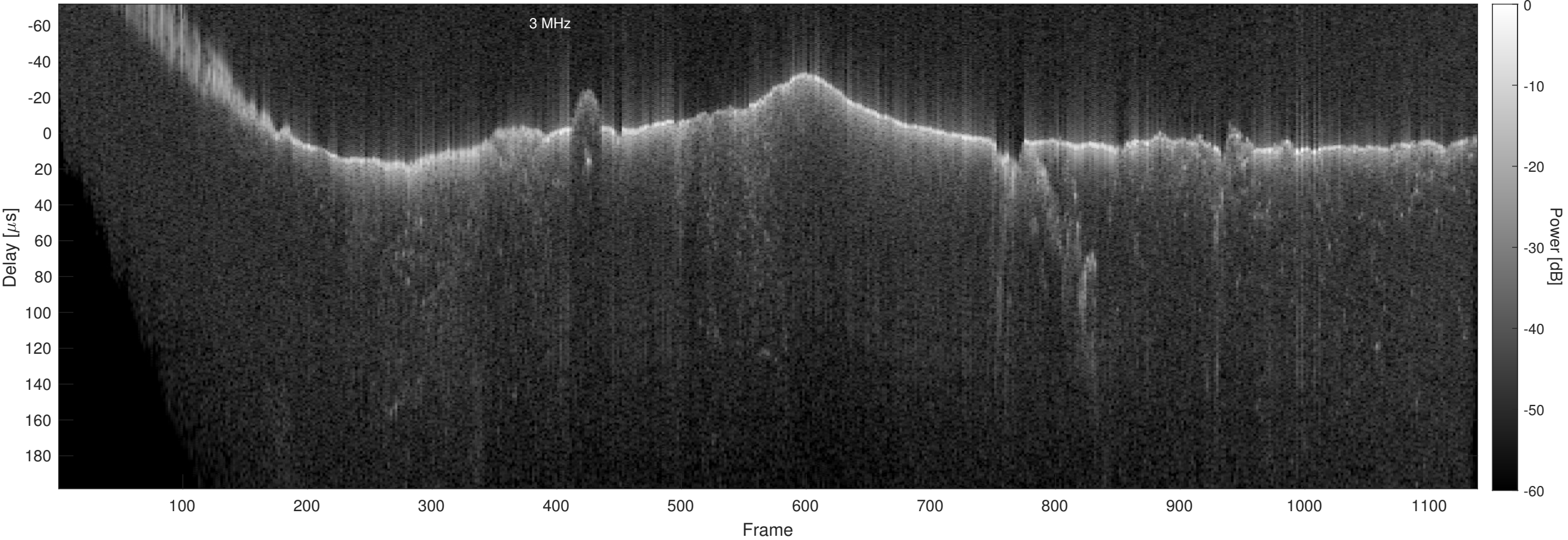
Orbit 17587, Chapman, No Window, Channel 2
