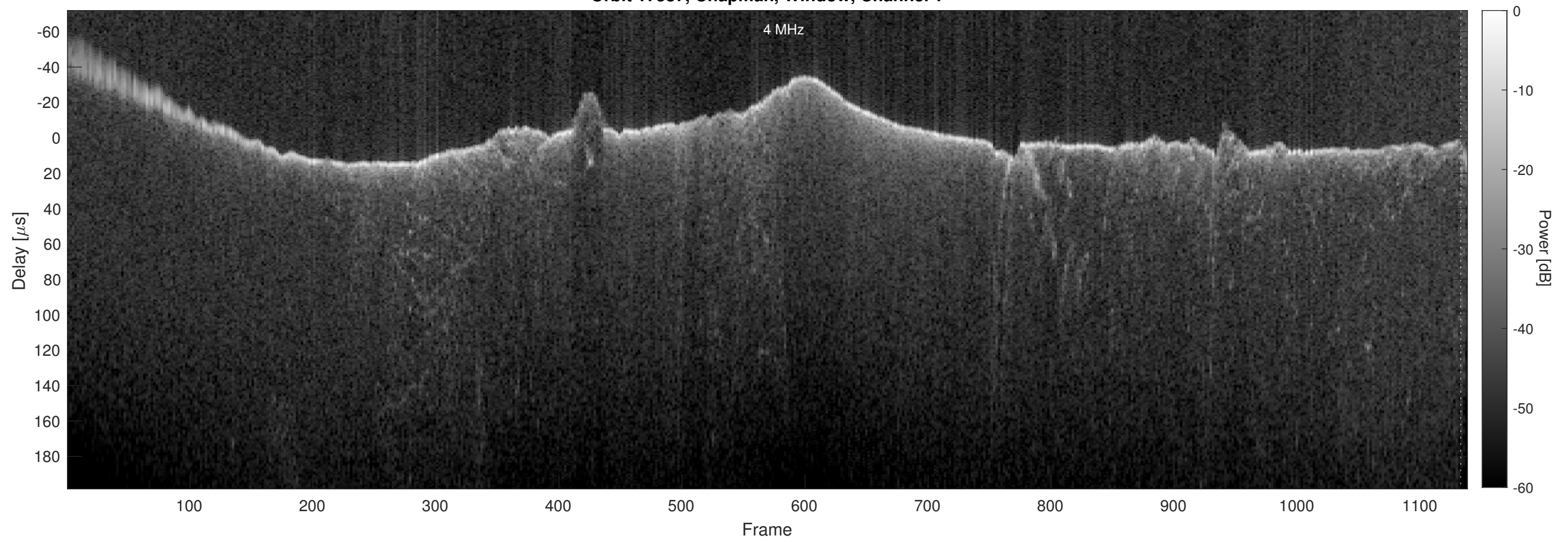
Orbit 17587, Chapman, Window, Channel 2
