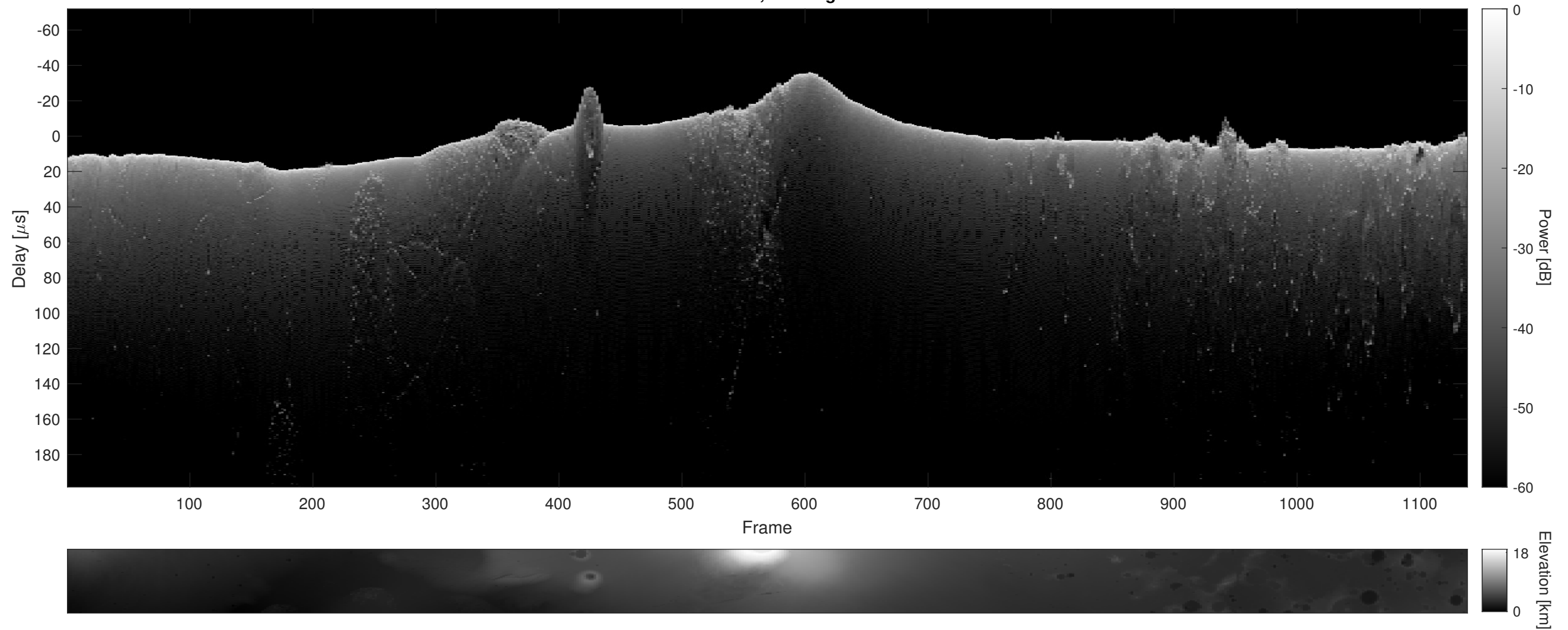
Orbit 17587, Cluttergram
