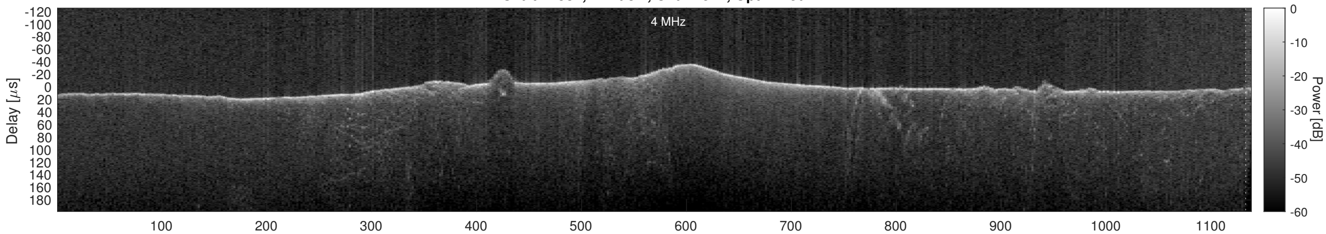
Orbit 17587, Cluttergram
