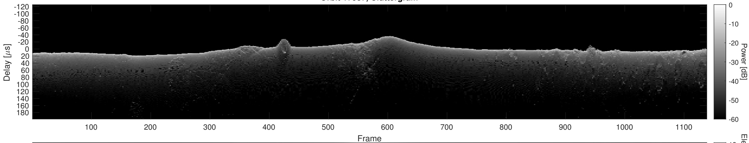
Orbit 17587, Cluttergram
