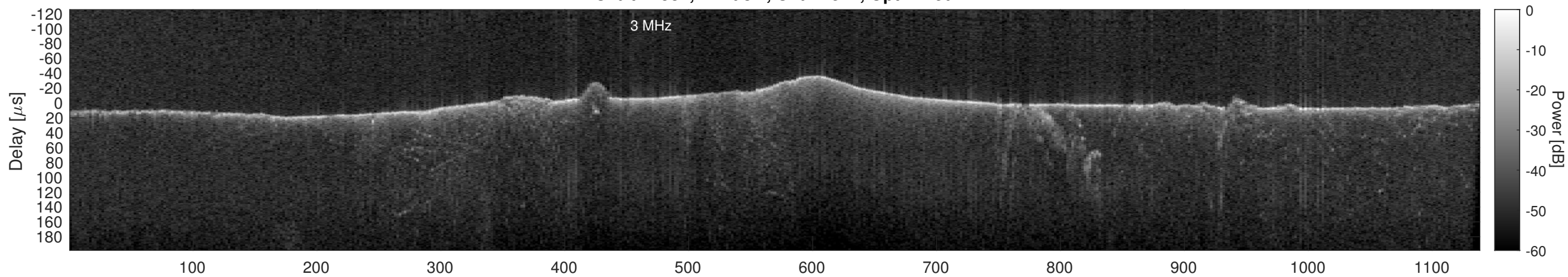
Orbit 17587, Cluttergram
