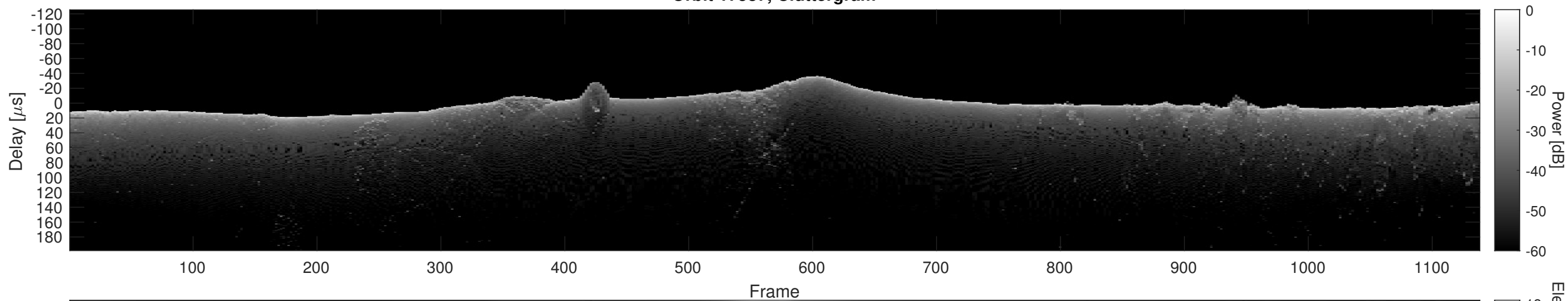
Orbit 17587, Cluttergram
