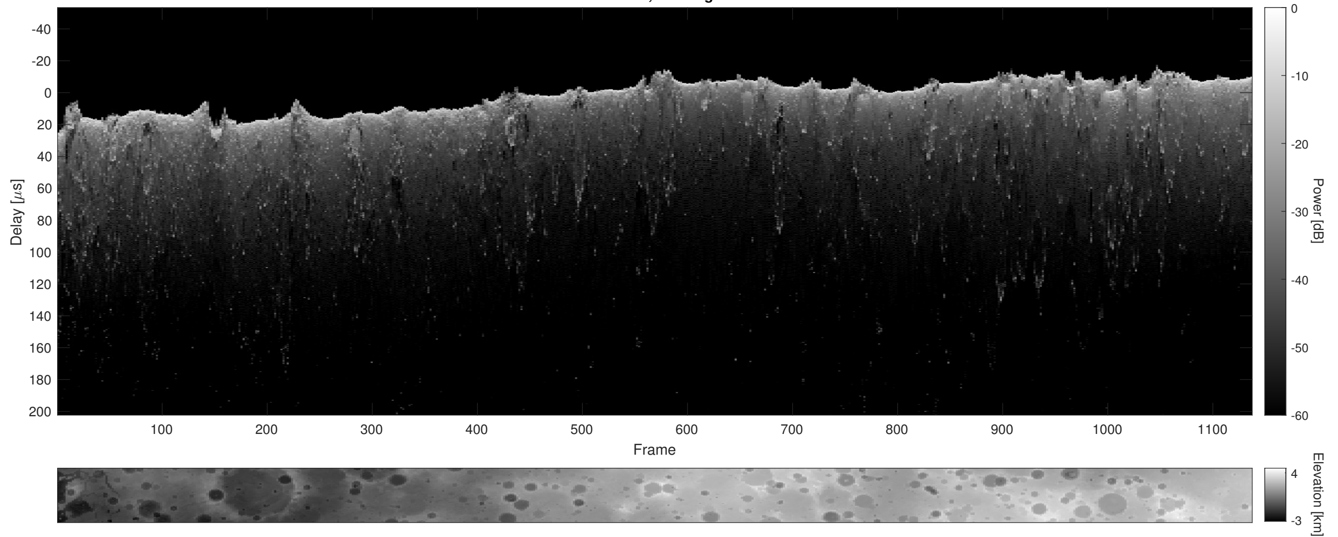
Orbit 17589, Cluttergram
