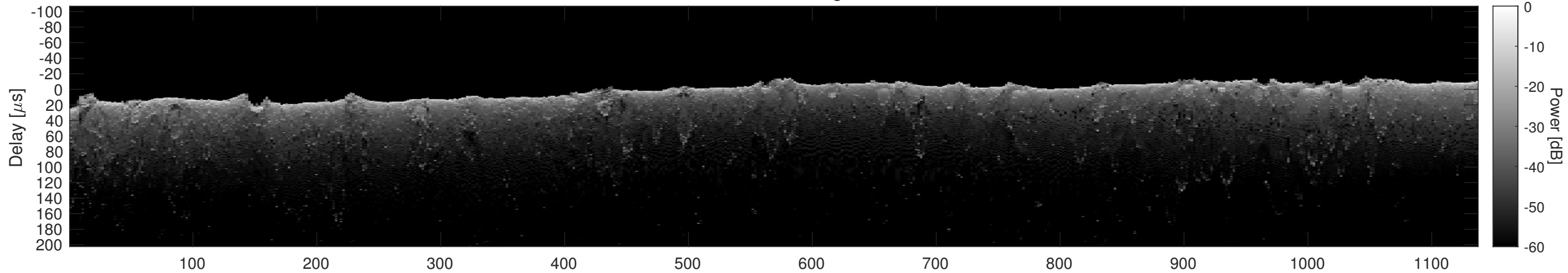
Orbit 17589, Cluttergram
