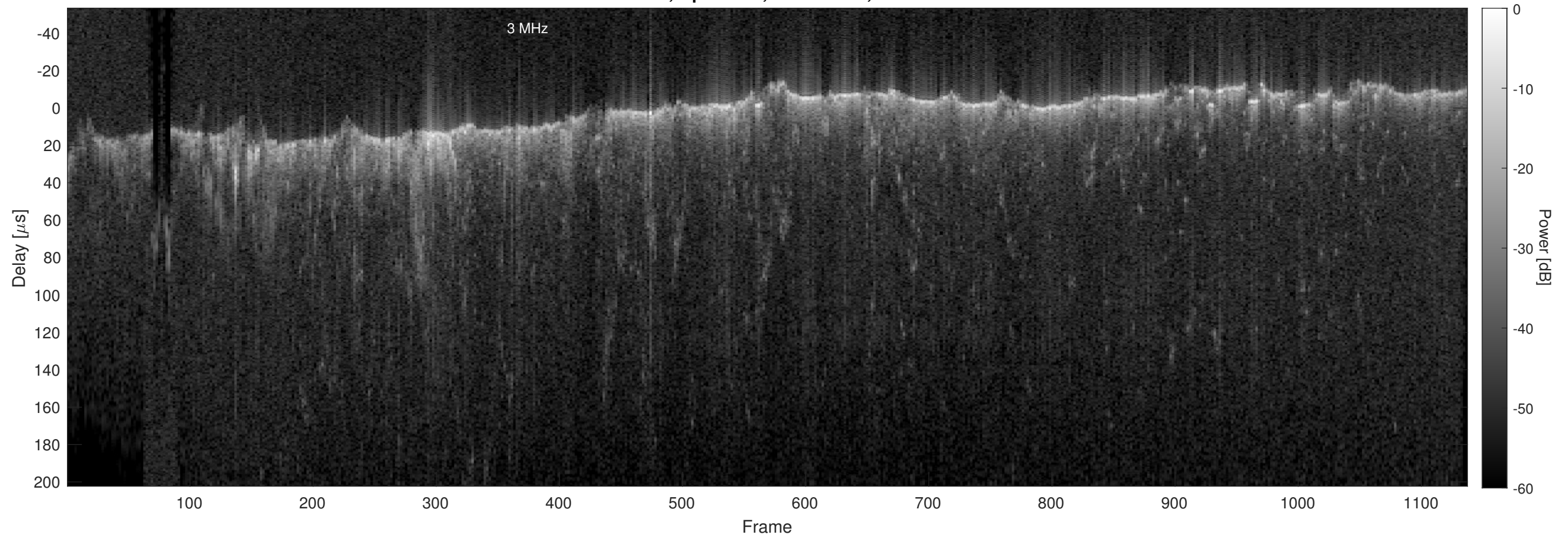
Orbit 17589, Optimized, No Window, Channel 2
