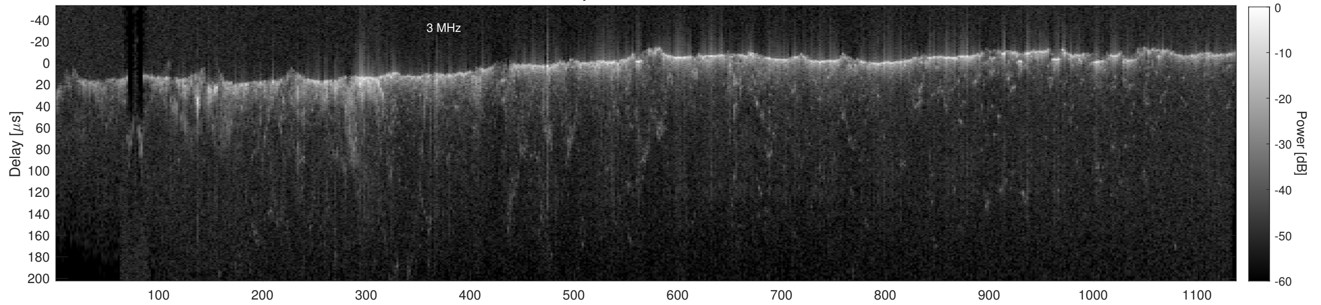
Orbit 17589, Cluttergram
