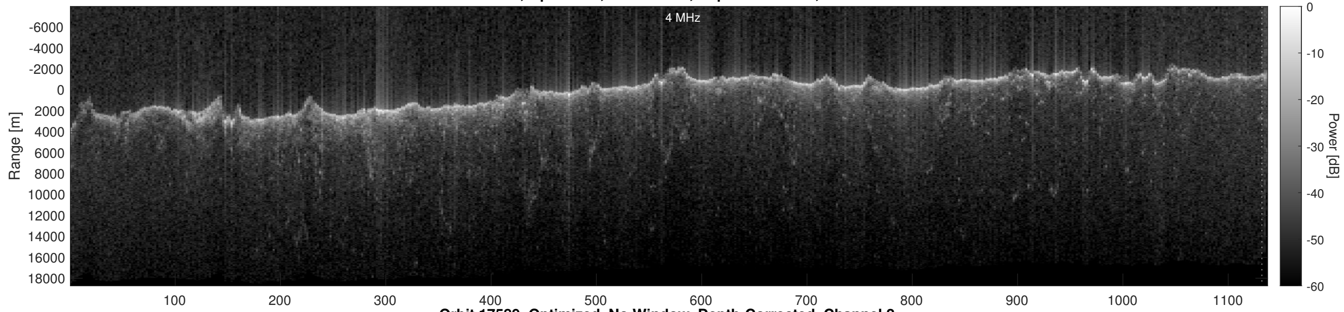
Orbit 17589, Optimized, No Window, Depth-Corrected, Channel 2
