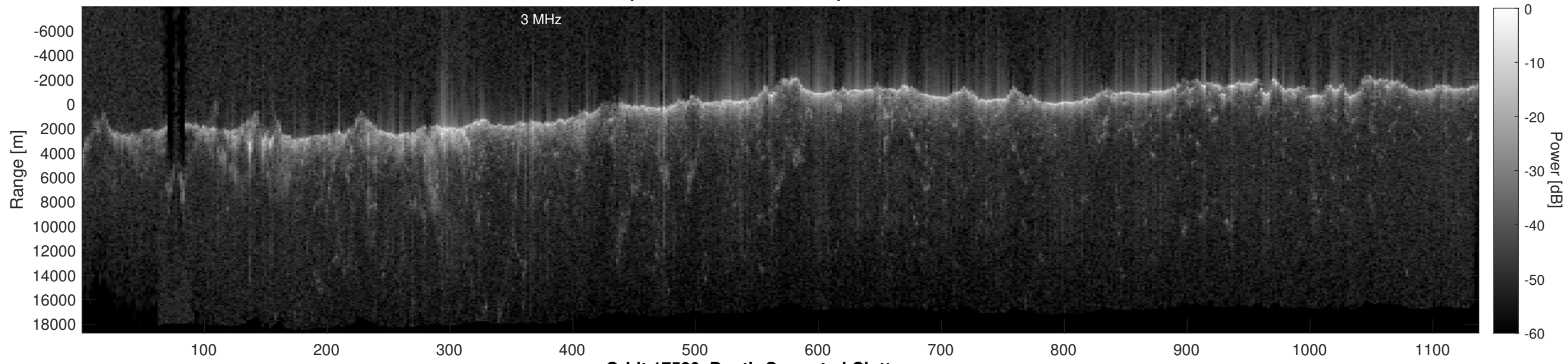
Orbit 17589, Depth-Corrected Cluttergram
