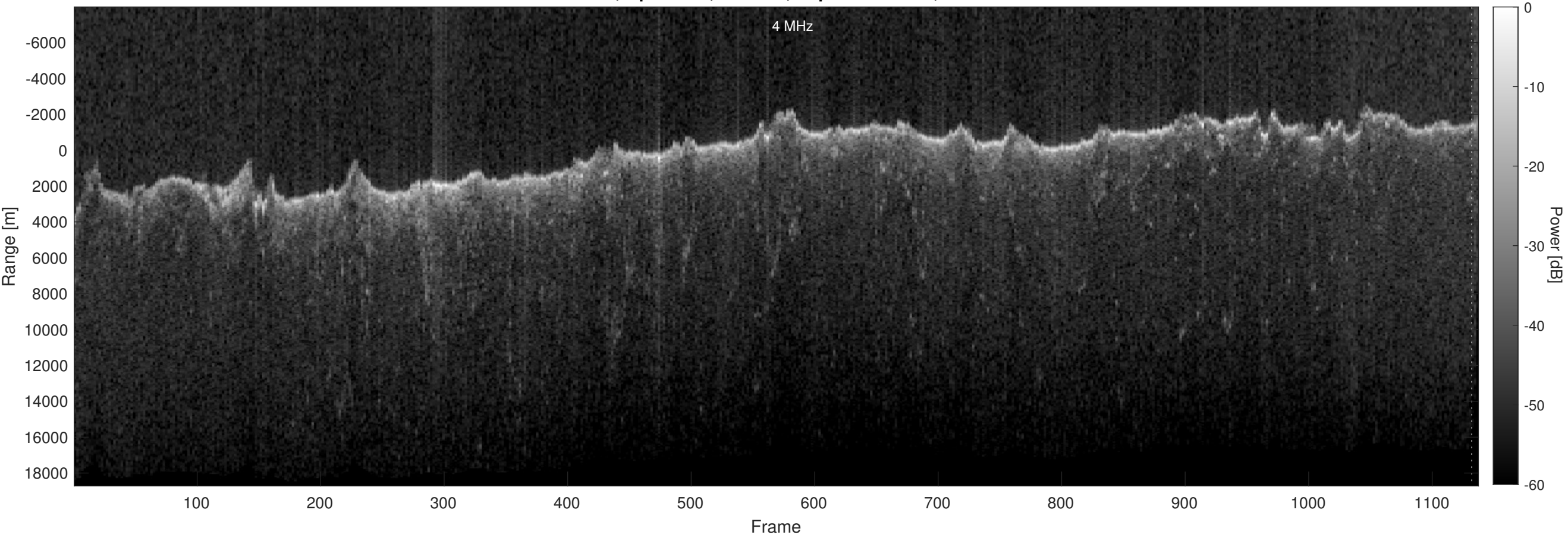
Orbit 17589, Optimized, Window, Depth-Corrected, Channel 2
