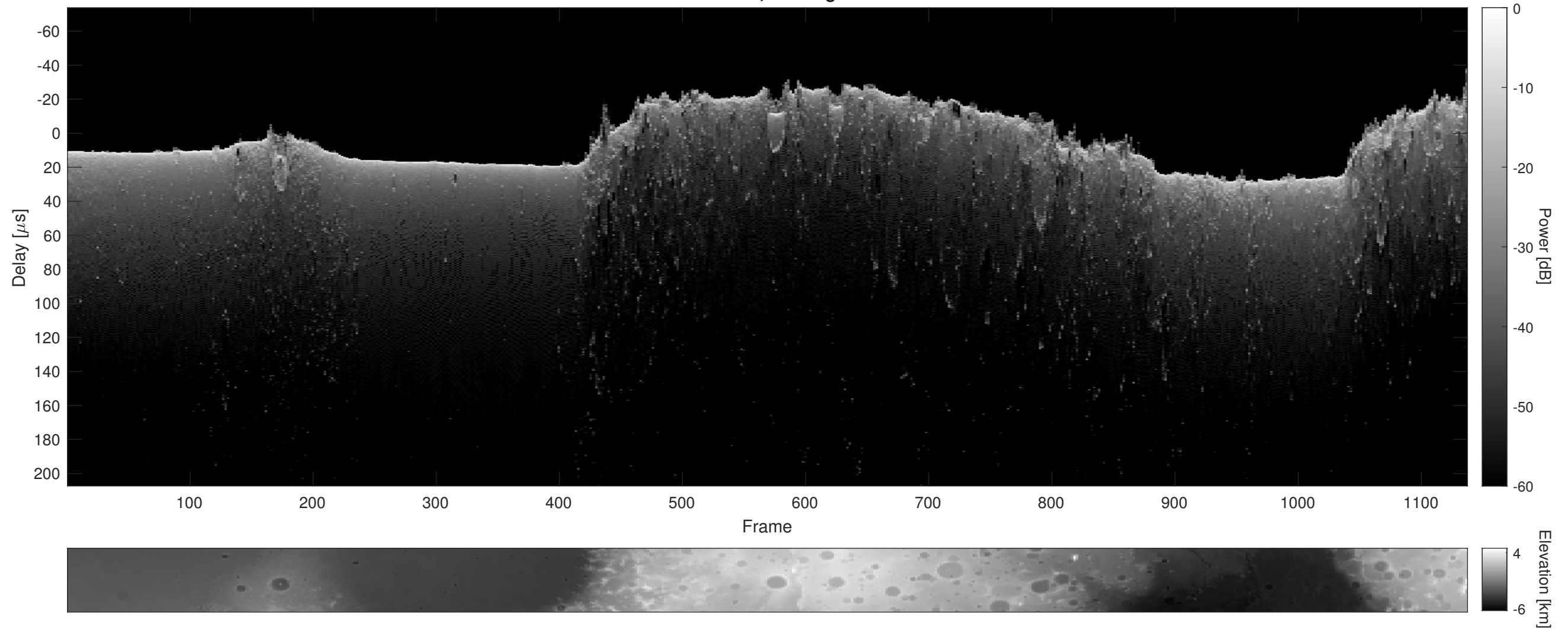
Orbit 17592, Cluttergram
