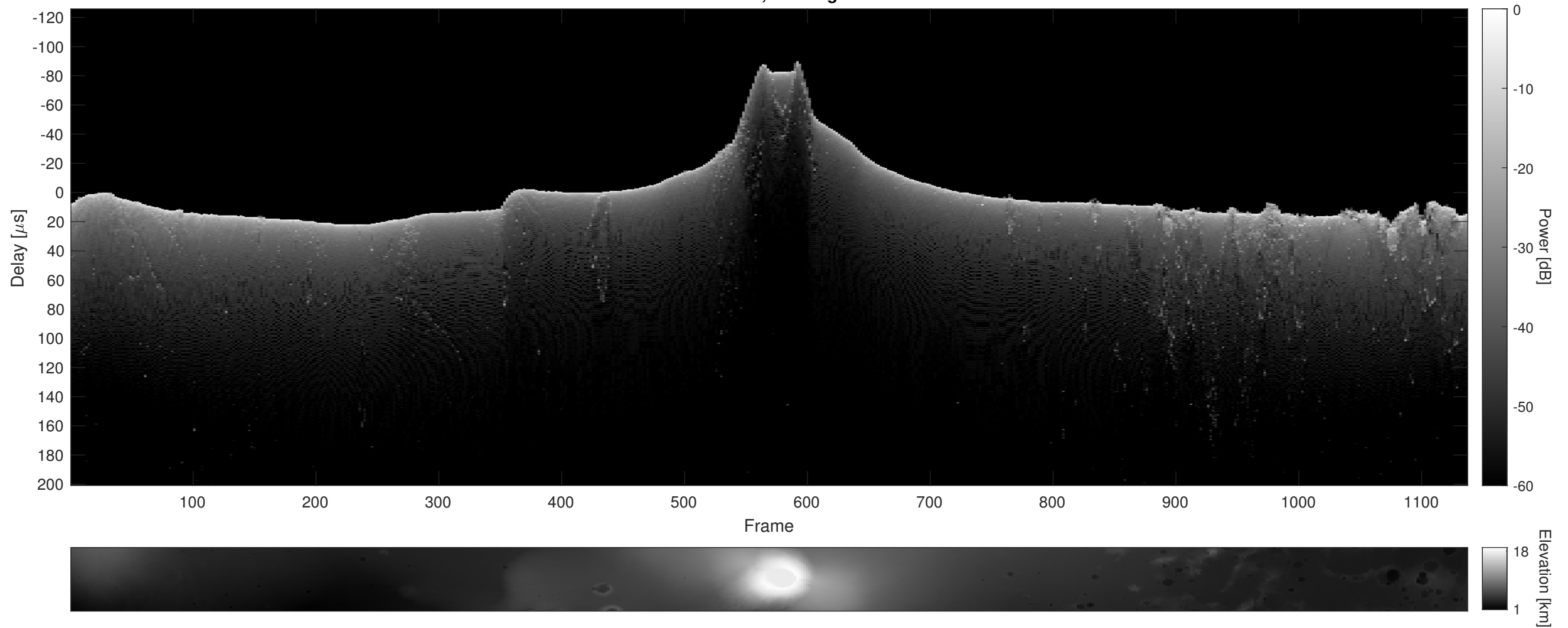
Orbit 17594, Cluttergram
