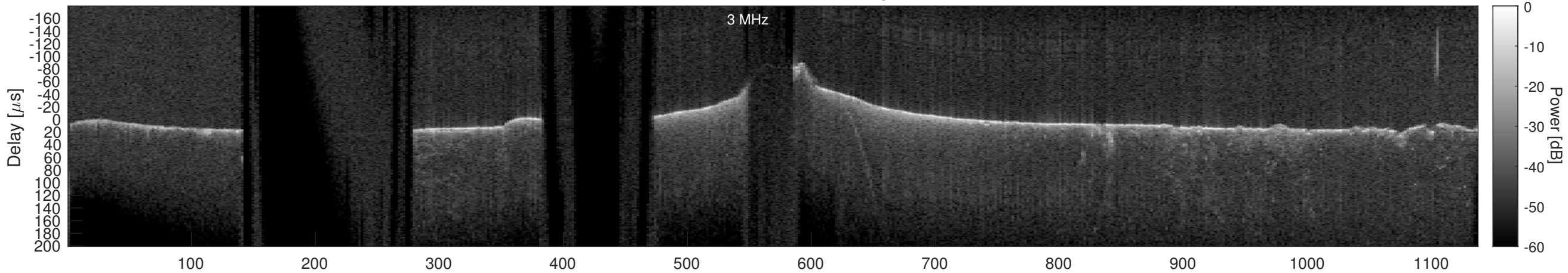
Orbit 17594, Cluttergram
