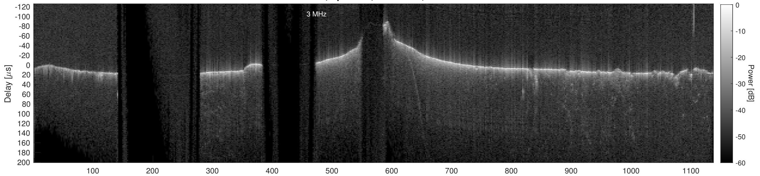
Orbit 17594, Cluttergram
