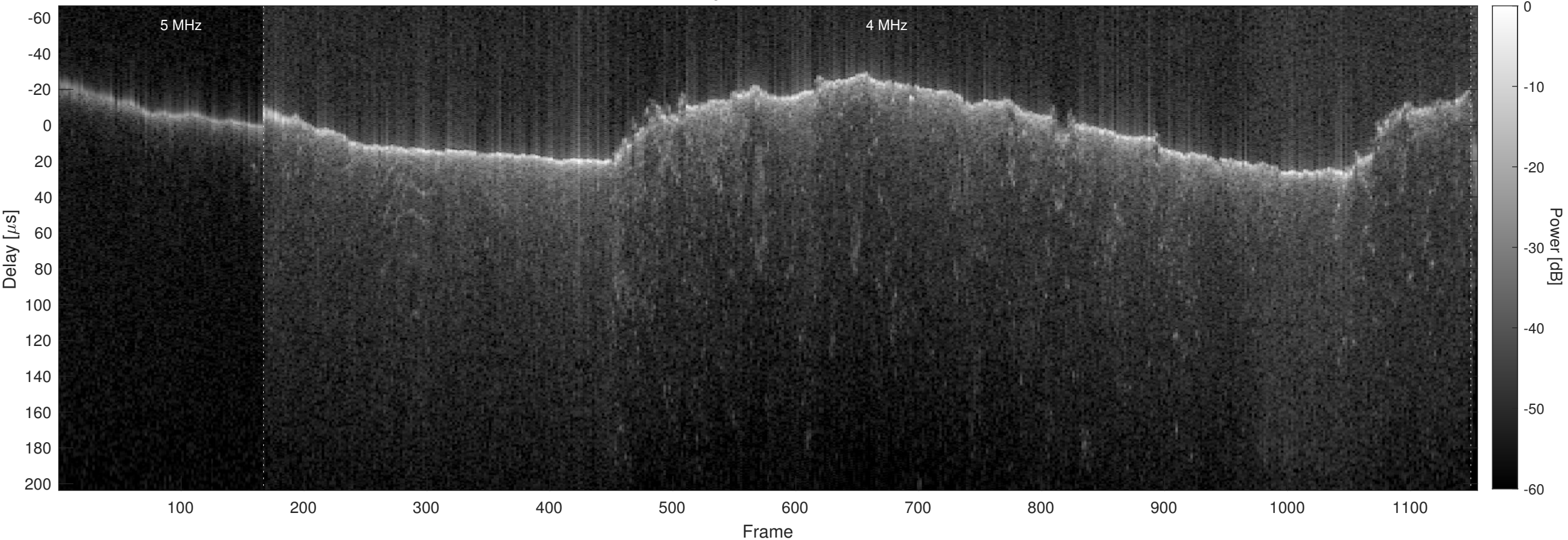
Orbit 17599, Chapman, No Window, Channel 2
