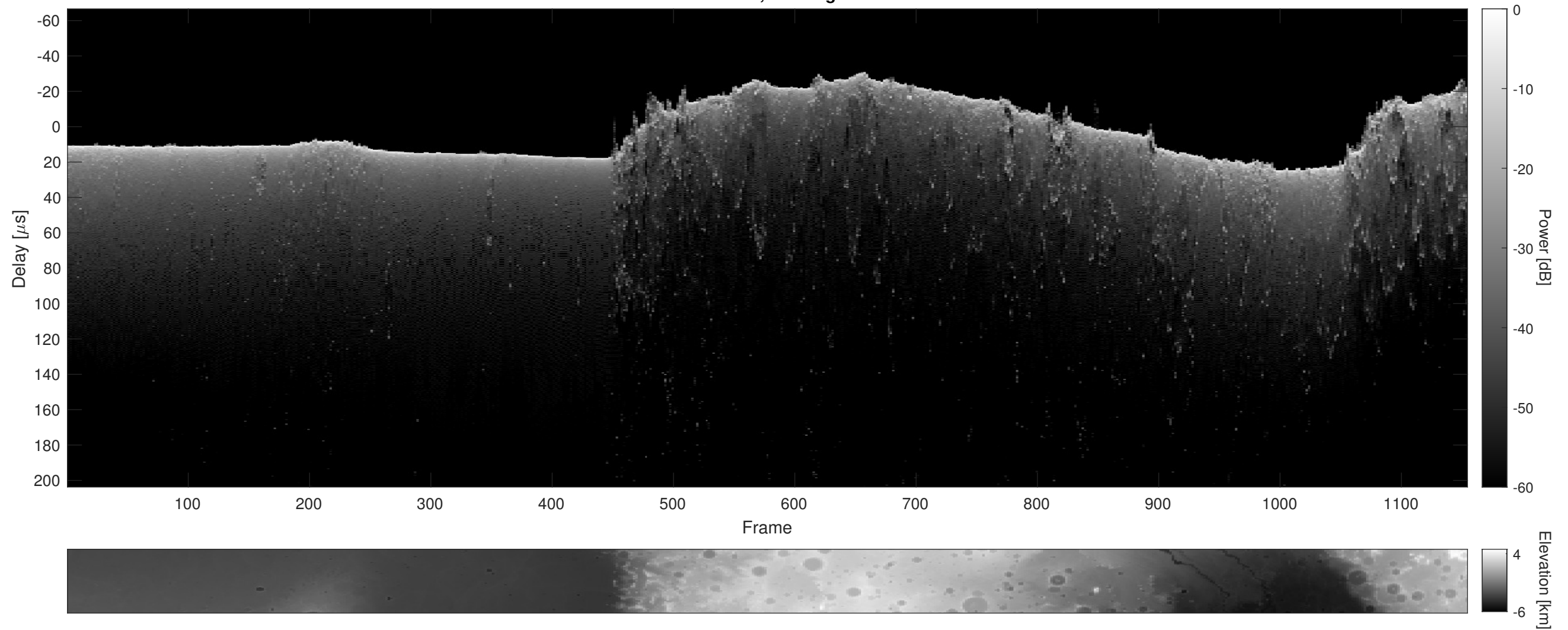
Orbit 17599, Cluttergram
