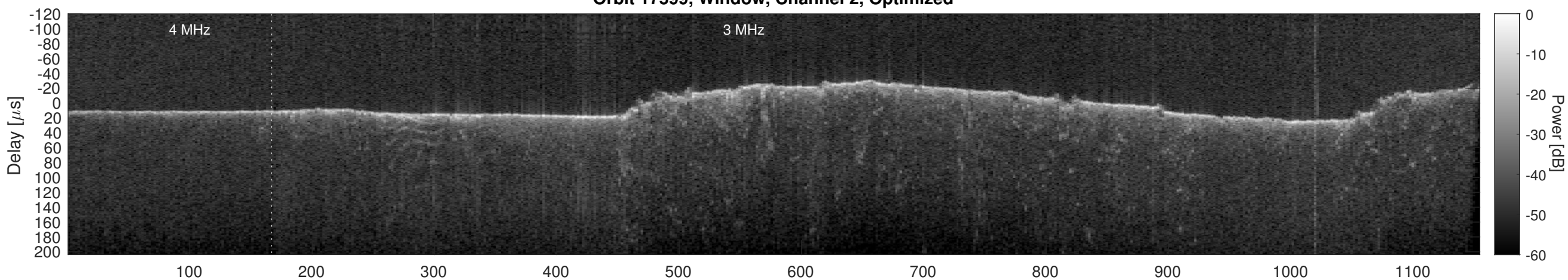
Orbit 17599, Cluttergram
