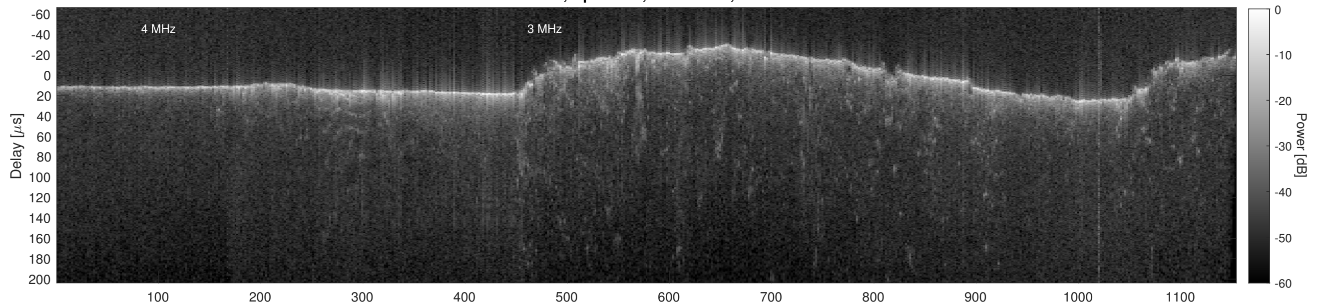
Orbit 17599, Cluttergram
