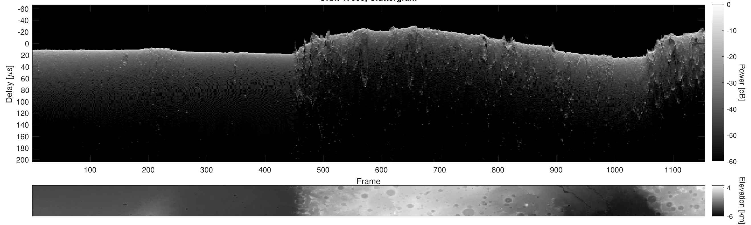
Orbit 17599, Cluttergram
