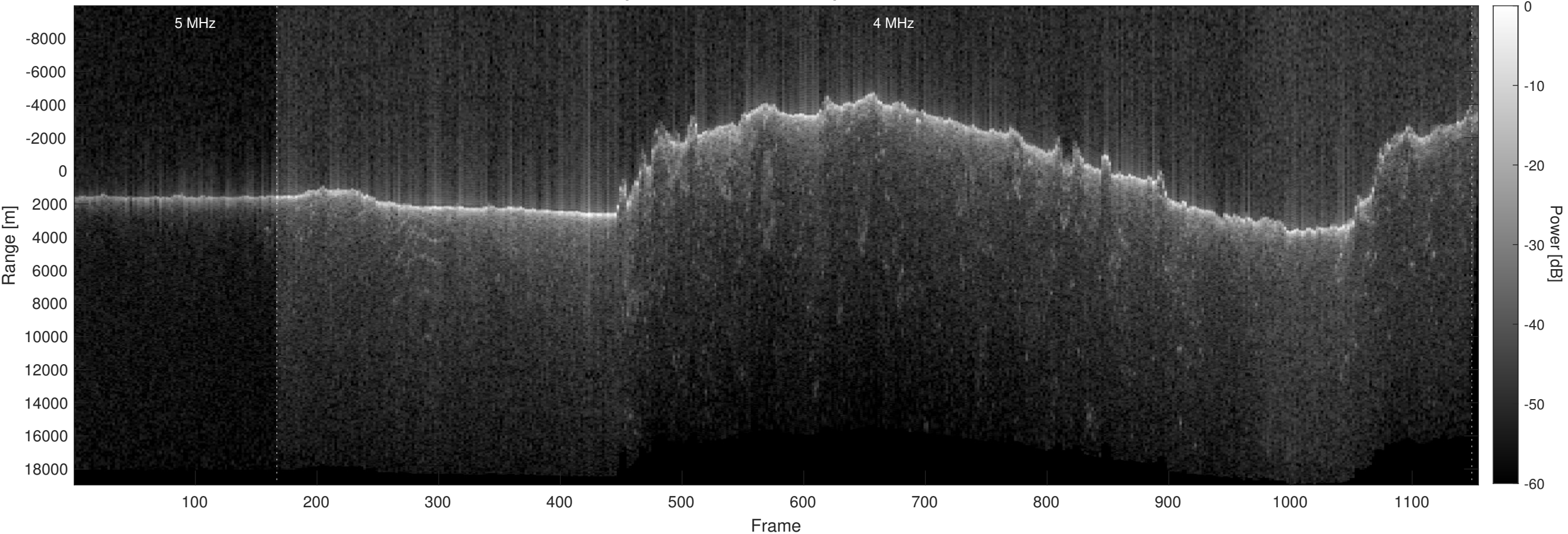
Orbit 17599, Optimized, No Window, Depth-Corrected, Channel 2
