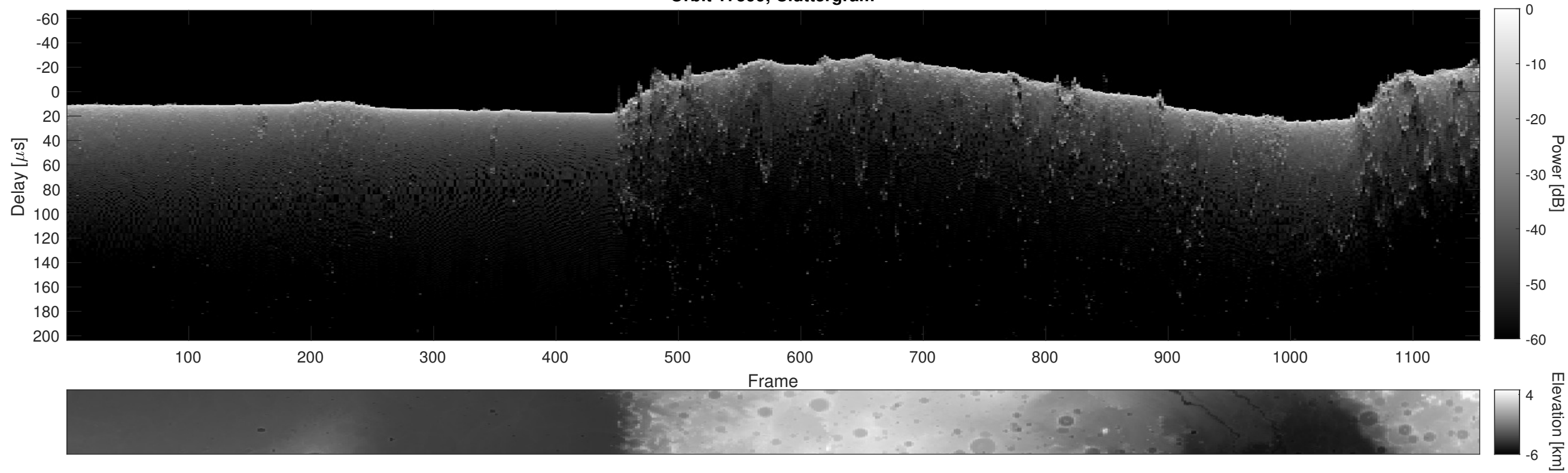
Orbit 17599, Cluttergram
