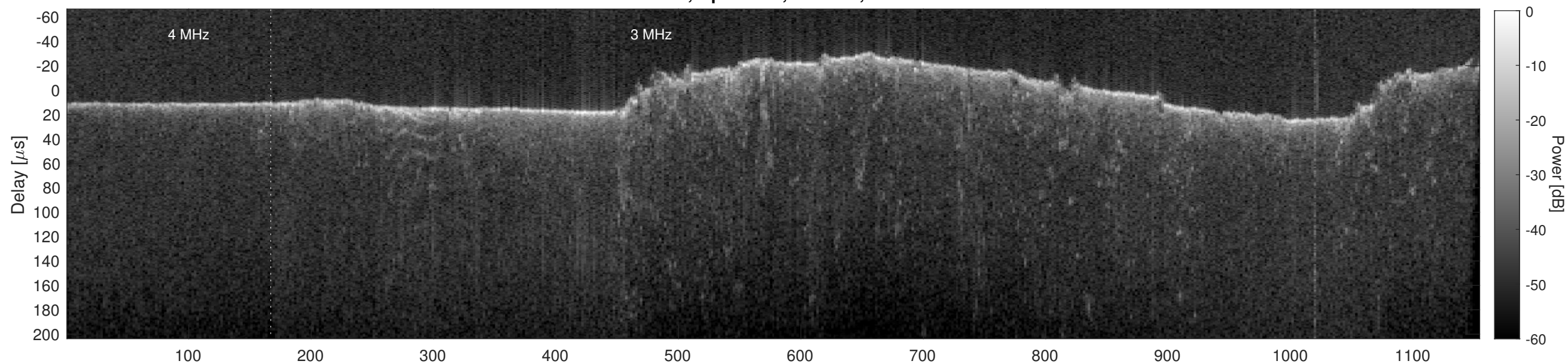
Orbit 17599, Cluttergram
