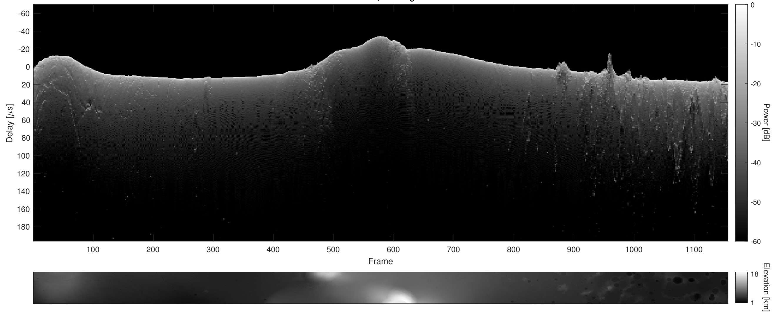
Orbit 17601, Cluttergram
