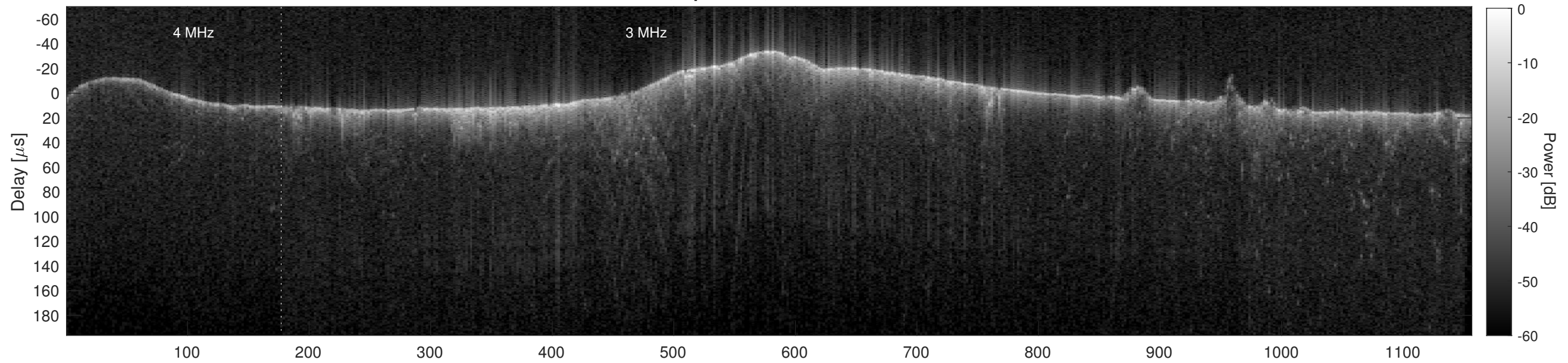
Orbit 17601, Cluttergram
