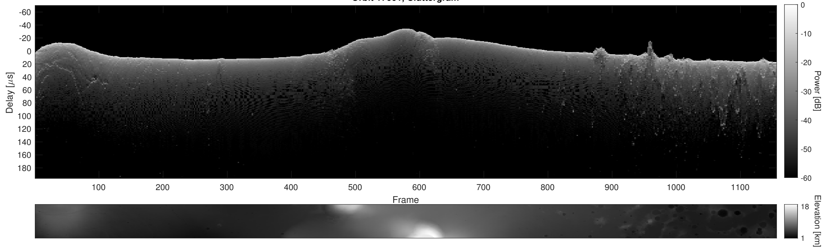
Orbit 17601, Cluttergram
