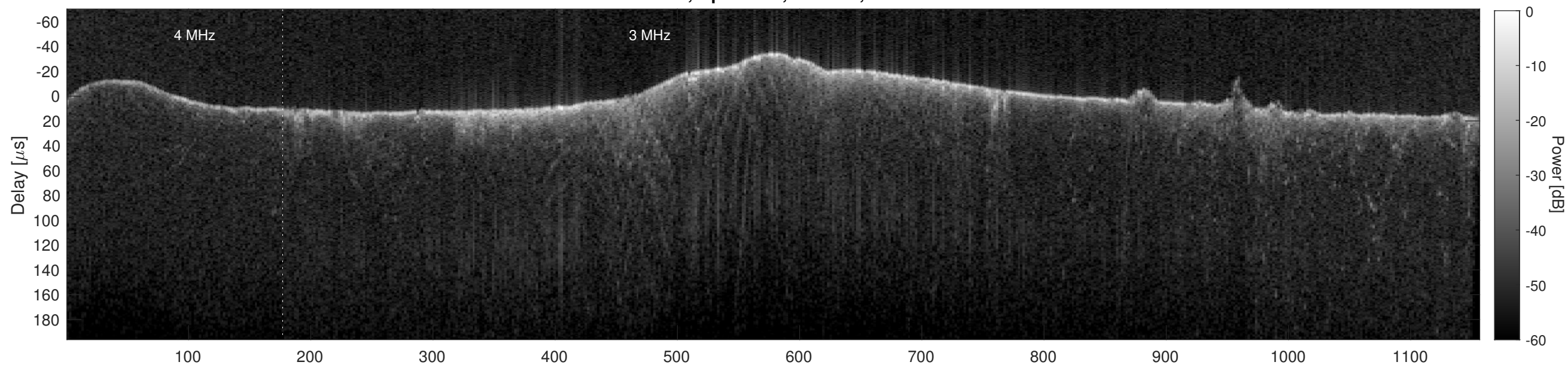
Orbit 17601, Cluttergram
