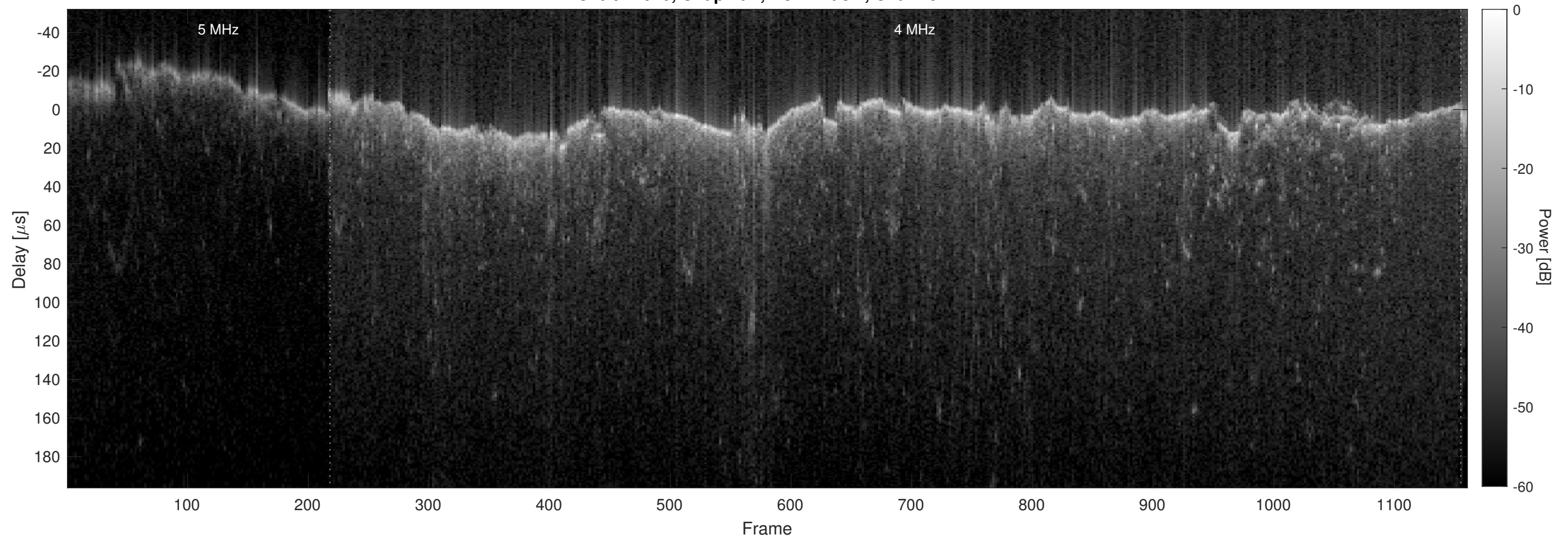
Orbit 17610, Chapman, No Window, Channel 2
