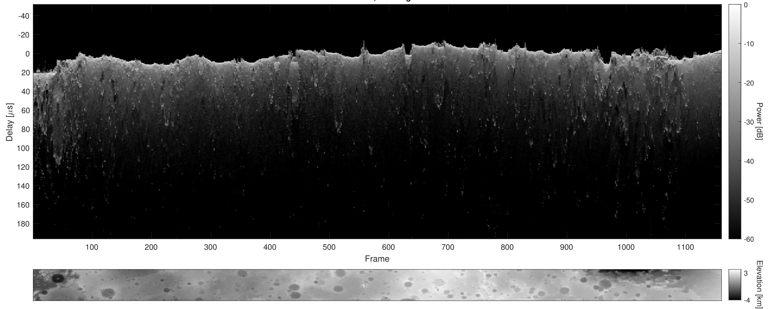
Orbit 17610, Cluttergram
