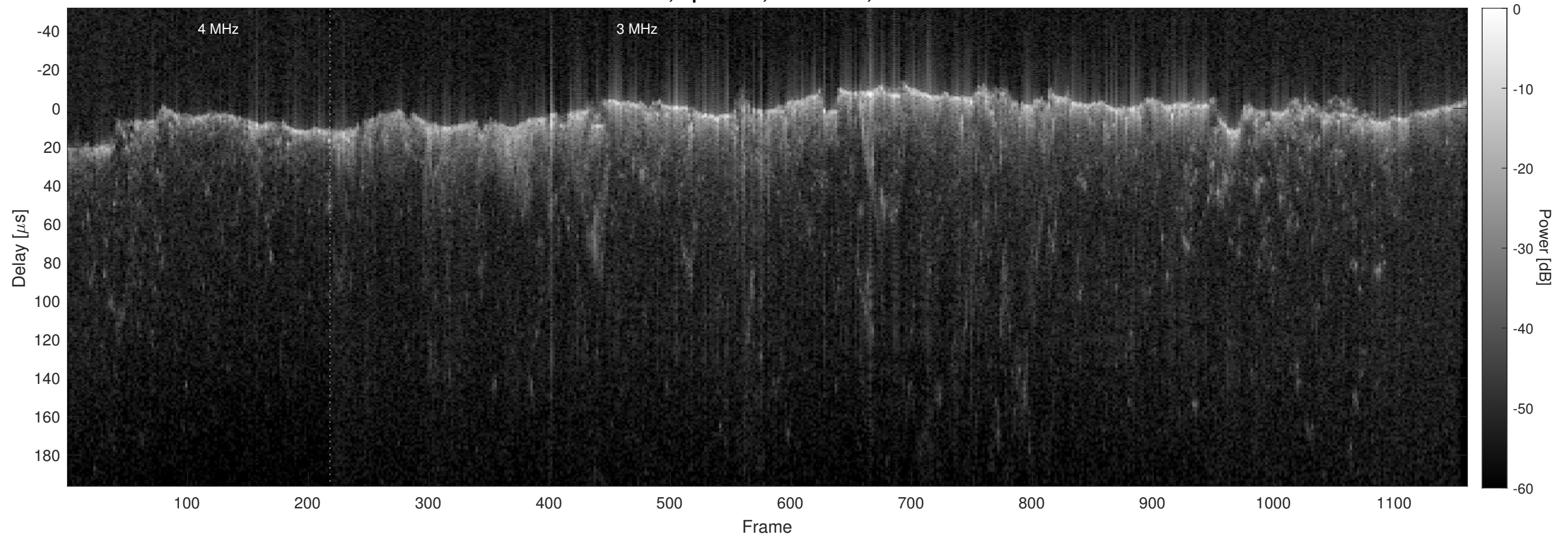
Orbit 17610, Optimized, No Window, Channel 2
