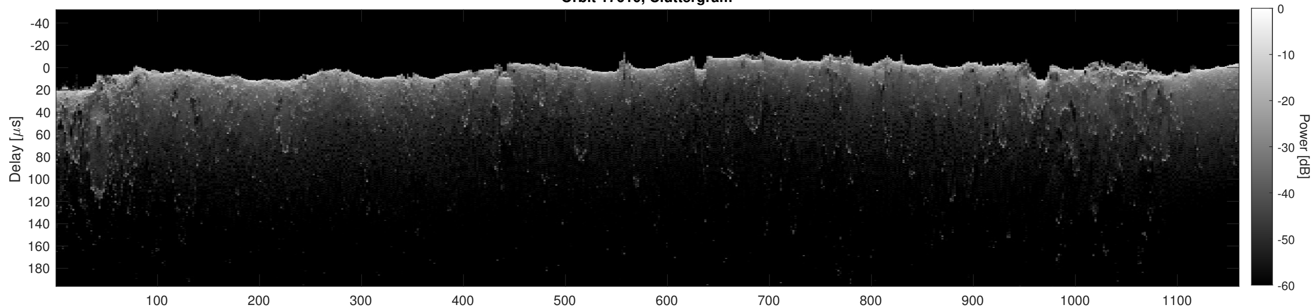
Orbit 17610, Cluttergram
