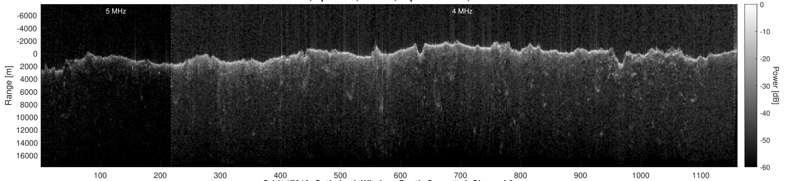
Orbit 17610, Optimized, Window, Depth-Corrected, Channel 2
