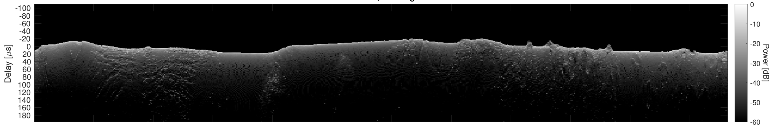
Orbit 17615, Cluttergram
