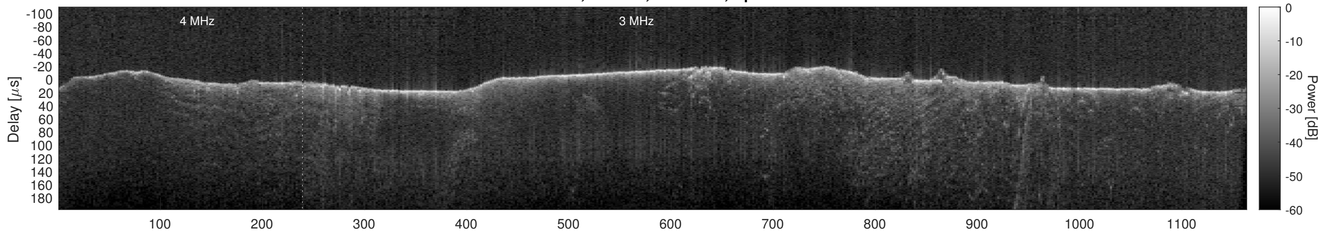
Orbit 17615, Cluttergram
