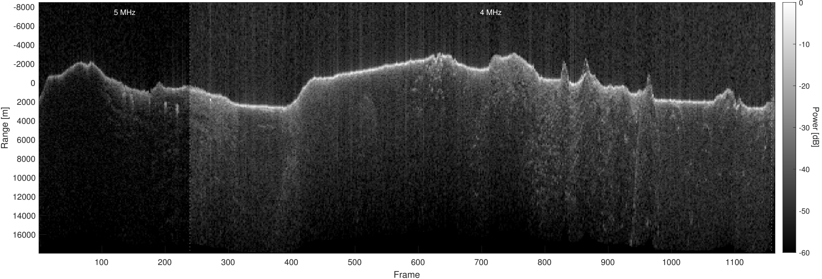
Orbit 17615, Optimized, Window, Depth-Corrected, Channel 2
