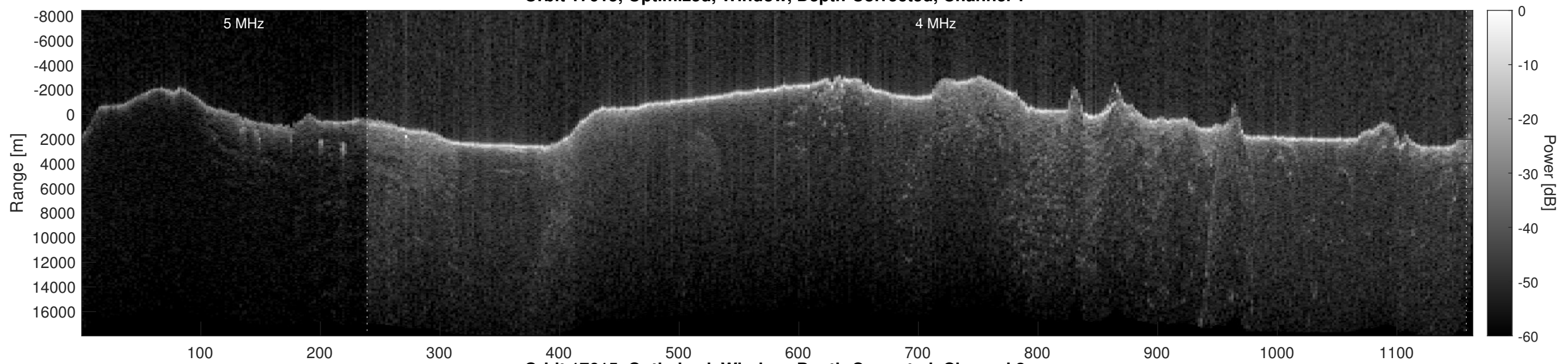
Orbit 17615, Optimized, Window, Depth-Corrected, Channel 2
