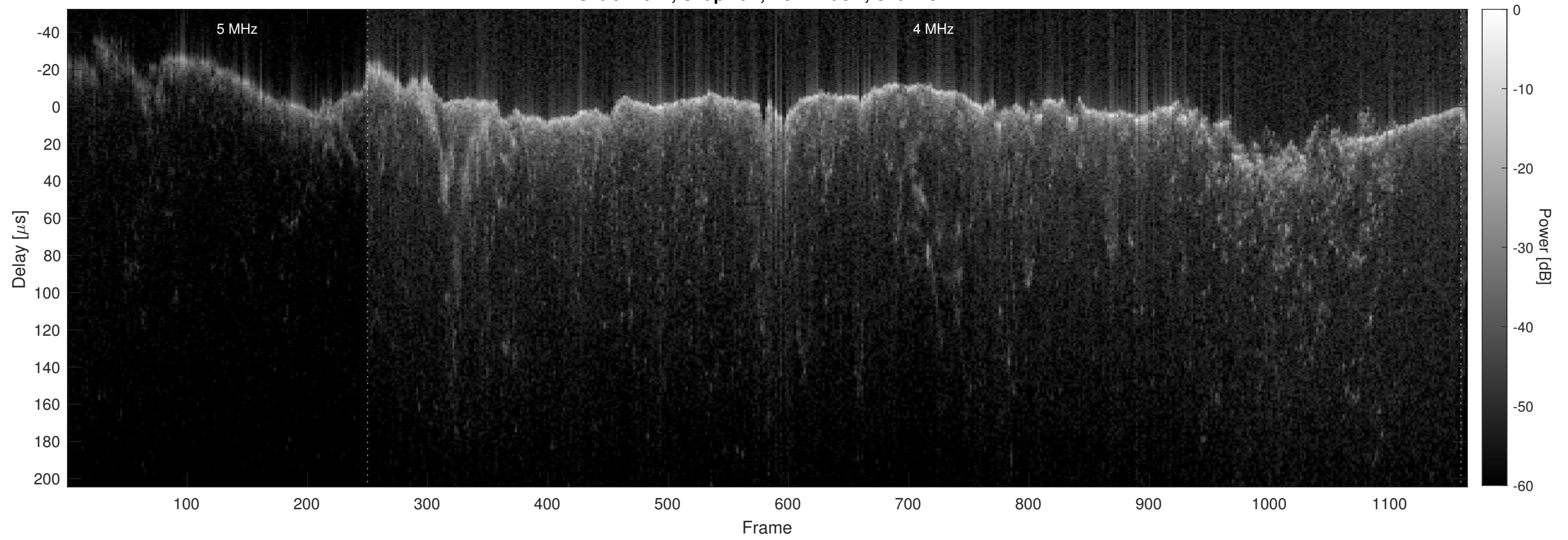
Orbit 17617, Chapman, No Window, Channel 2
