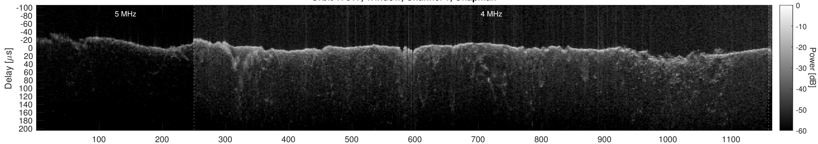
Orbit 17617, Window, Channel 1, Optimized
