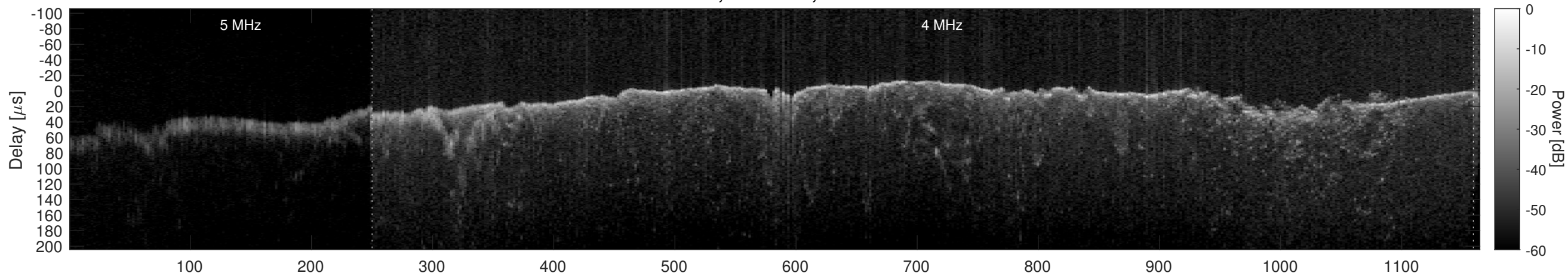
Orbit 17617, Window, Channel 1, Chapman
