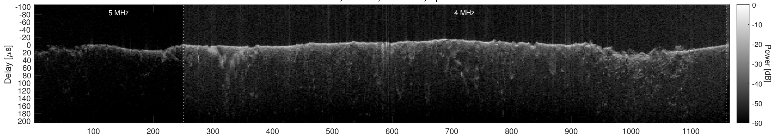
Orbit 17617, Cluttergram
