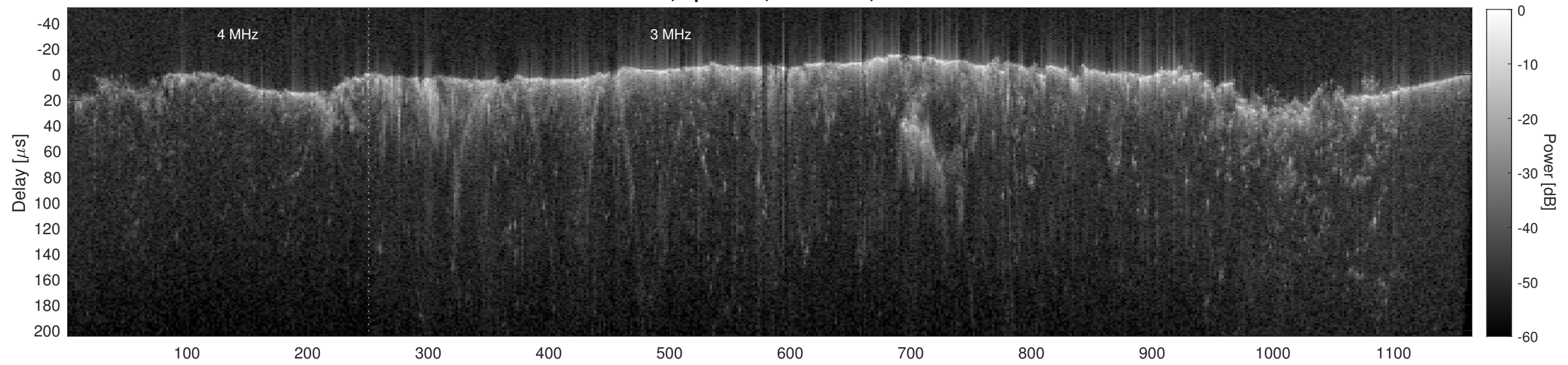
Orbit 17617, Cluttergram
