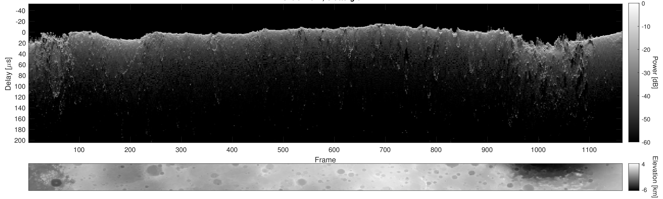
Orbit 17617, Cluttergram
