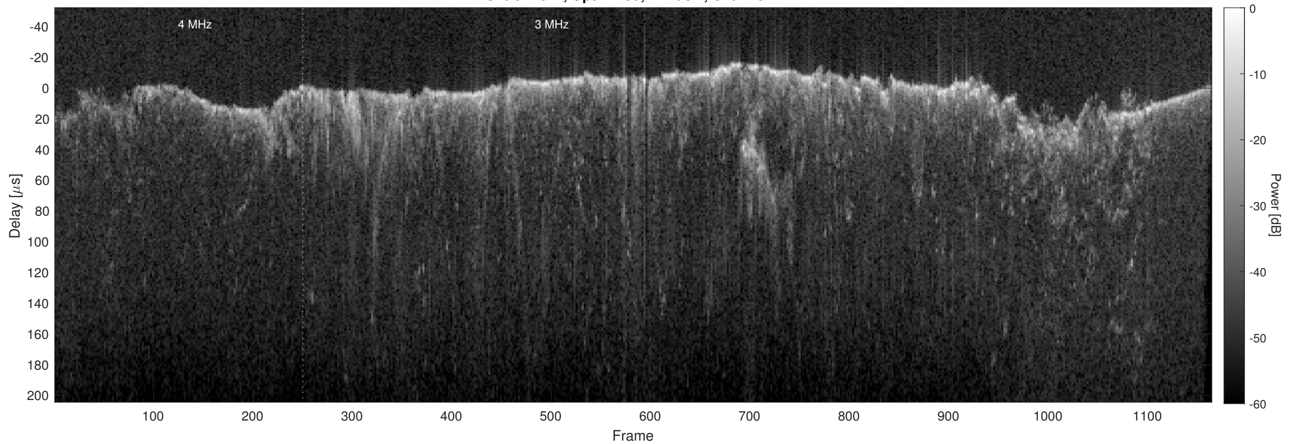
Orbit 17617, Optimized, Window, Channel 2
