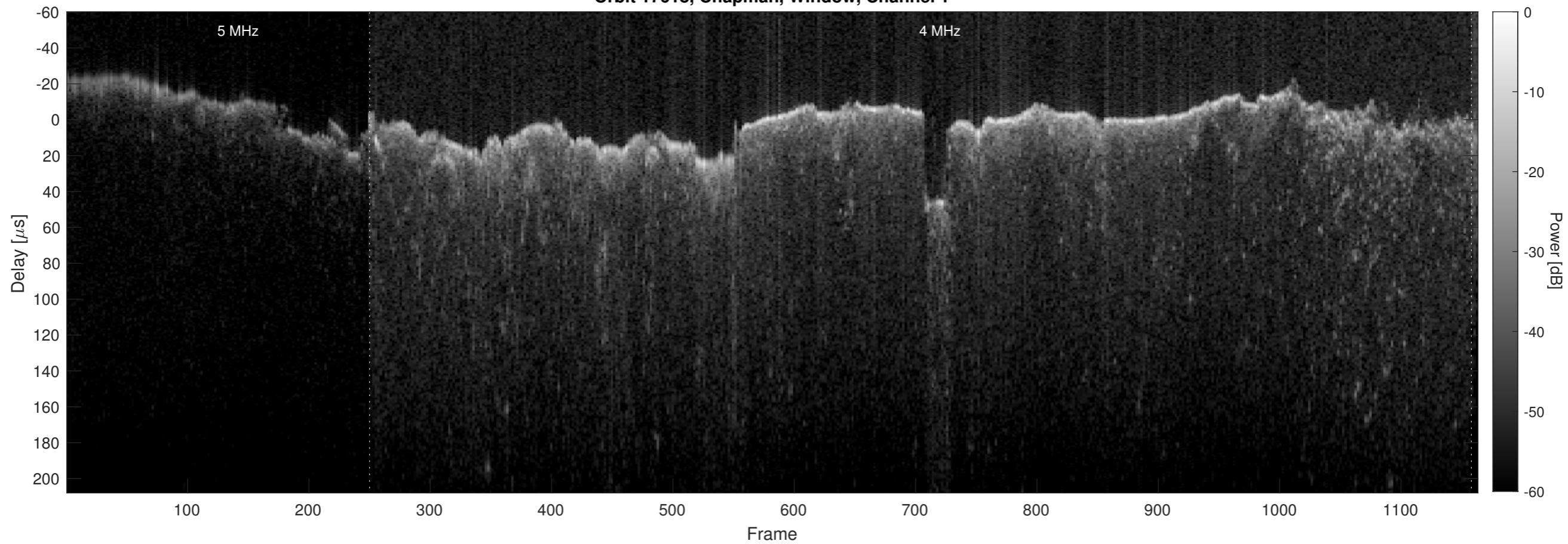
Orbit 17618, Chapman, Window, Channel 2
