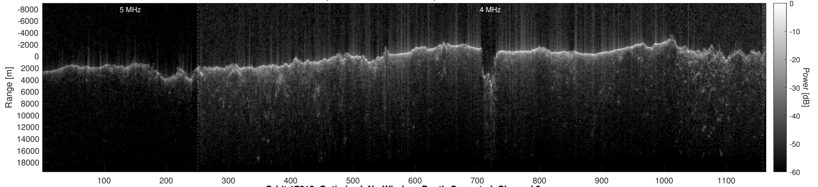
Orbit 17618, Optimized, No Window, Depth-Corrected, Channel 2
