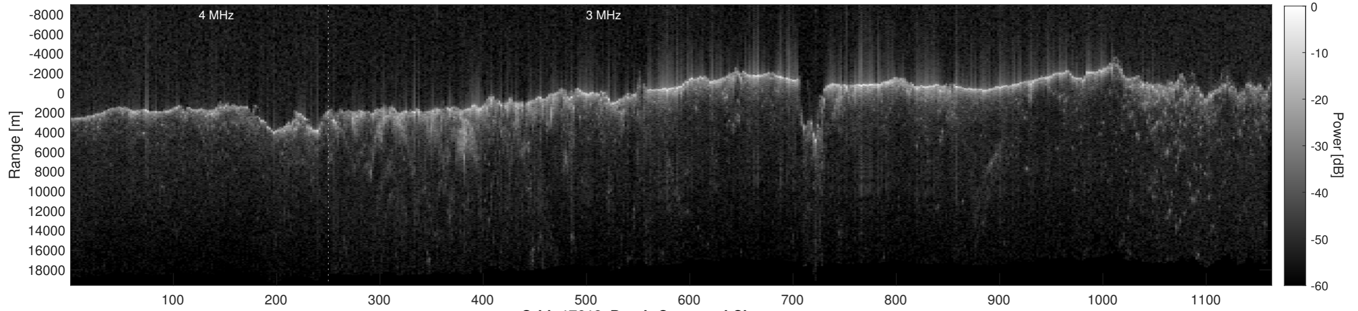
Orbit 17618, Depth-Corrected Cluttergram
