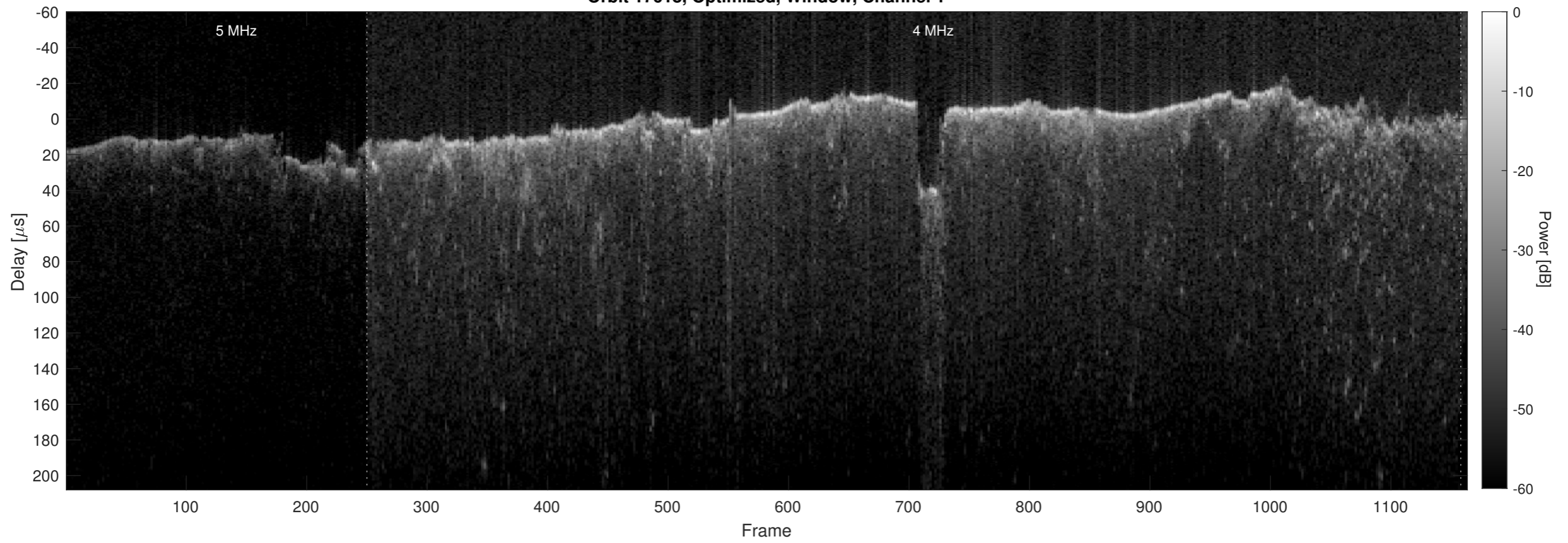
Orbit 17618, Optimized, Window, Channel 2
