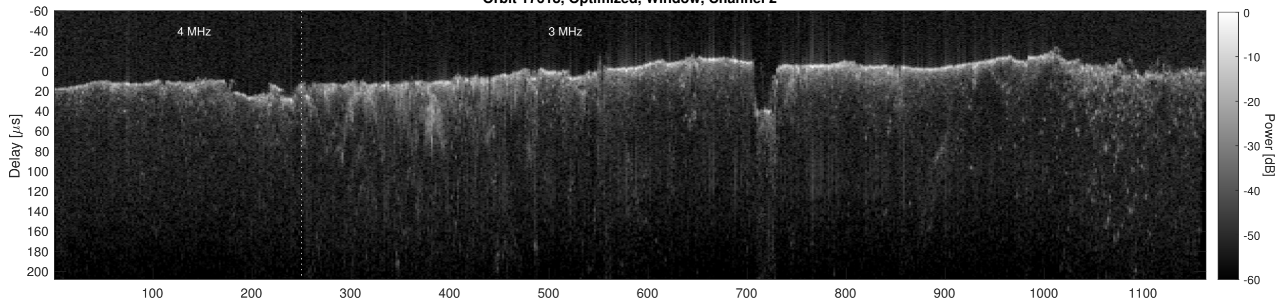
Orbit 17618, Cluttergram
